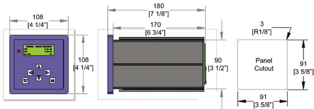
Dimensions Diagram
